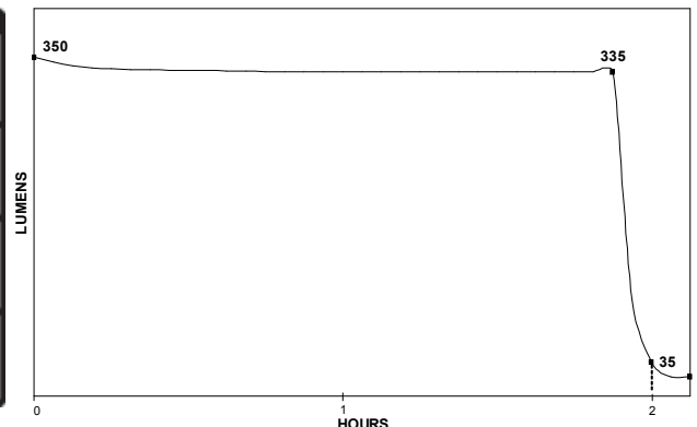
SL-20L / SL-20LP PERFORMANCE CURVE
