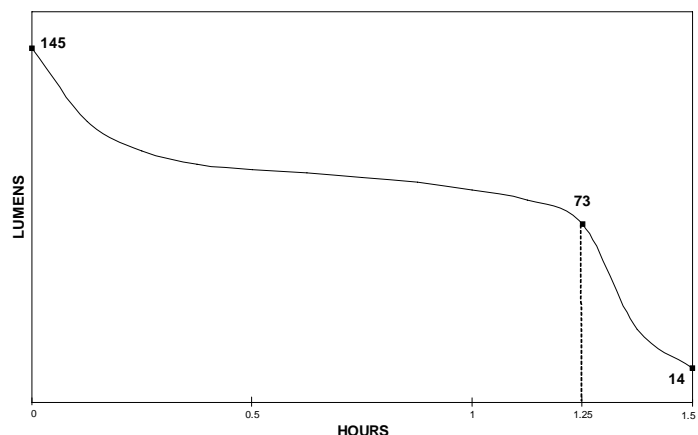
SL-20XP PERFORMANCE CURVE
